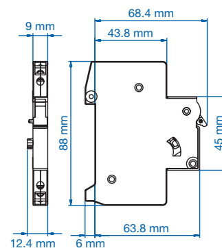
Dimensions HLS11M.
